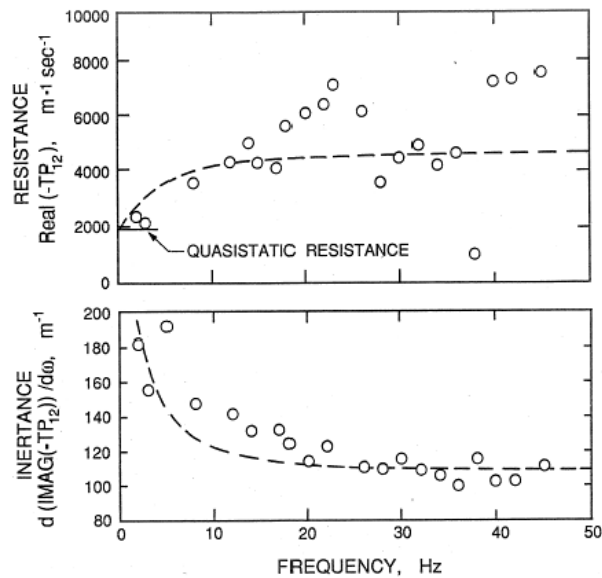
Figure 2: Typical inertance and resistance values from the centrifugal pump data of figure 1. Data do not include the diffuser contribution. The lines correspond to analytical values obtained as described in the text.
