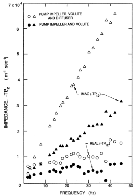
Figure 1: Impedance measurements made by Anderson, Blade and Stevans (1971) on a centrifugal pump (impeller diameter of 18.9 cm) operating at a flow coefficient of 0.442 and a speed of 3000 rpm. The real or resistive part of (-T_{12}) and the imaginary or reactive part of (T_{12}) are plotted against the frequency of the perturbation.
