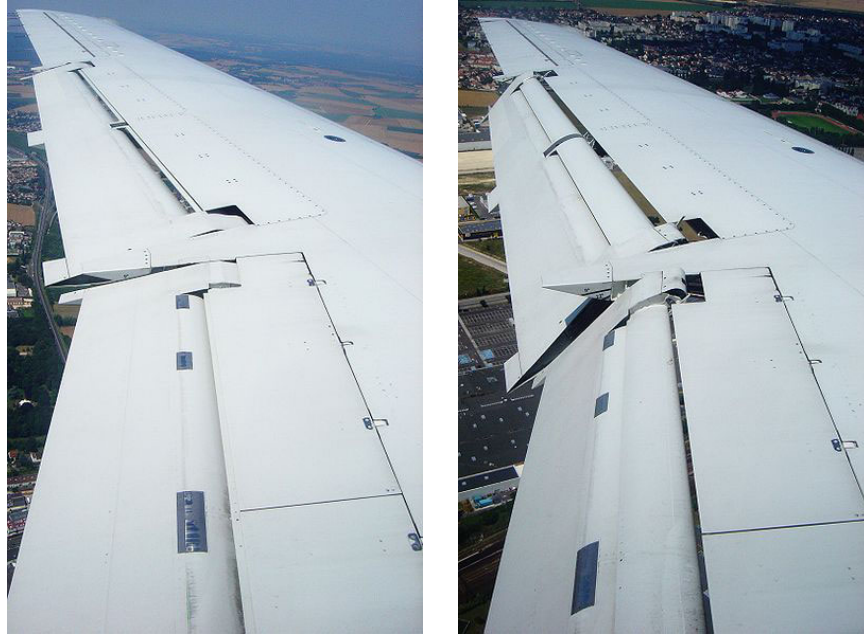
Figure 4: Wing of an Embraer ERJ 145 showing the flaps slightly extended (left) and fully extended (right).
