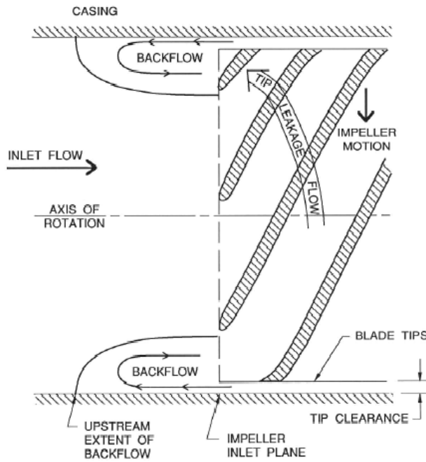
Figure 1: Lateral view of impeller inlet flow showing tip leakage flow leading to backflow.
