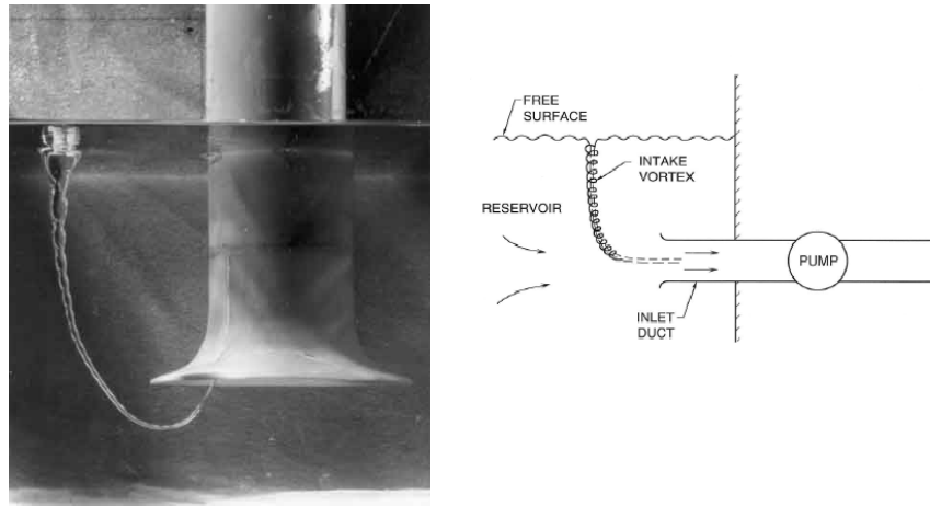
Figure 3: Right: sketch of a typical inlet vortex associated with prerotation. Left: Photograph of an air-filled inlet vortex from Wijdiëks (1965) reproduced with permission of the Delft Hydraulics Laboratory.
