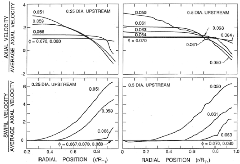
Figure 2: Axial and swirl velocity profiles in the inlet duct 0.25 diameters (left) and 0.5 diameters (right) upstream of the inlet plane of an inducer (Impeller VI) for various flow coefficients as shown (from del Valle, Braisted and Brennen 1992).
